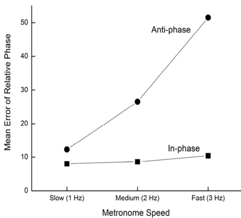
Fig. (2). Significant two-way interaction for phase x frequency ( F(1.49, 21)=41.69, p<.001 ). Mean error of relative phase as a function of frequency or metronome speed (i.e., slow (1Hz), medium (2Hz), and fast (3 Hz)) for the in-phase pattern and the anti-phase pattern.
