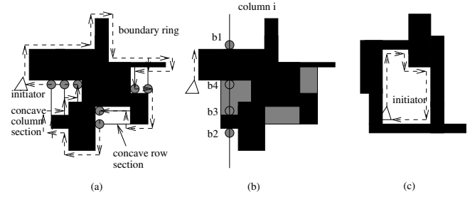
Figure 5. Distributed solution for (a) and (b) open concave region, and for (c) closed concave region.
